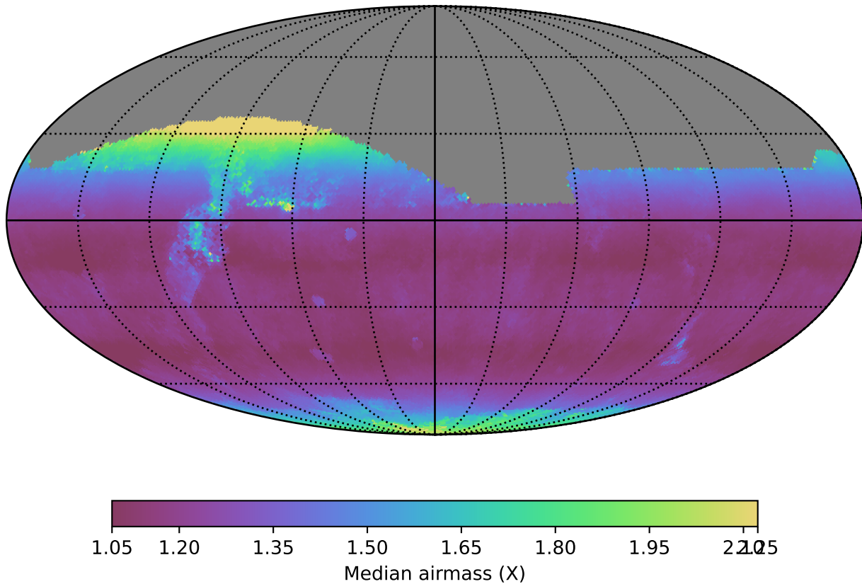
baseline_v3.5_10yrs All sky z band: Median airmass
