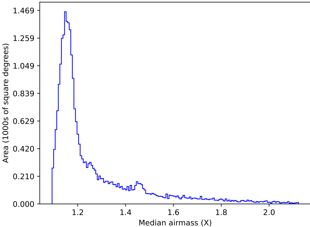
baseline_v3.5_10yrs All sky z band: Median airmass
