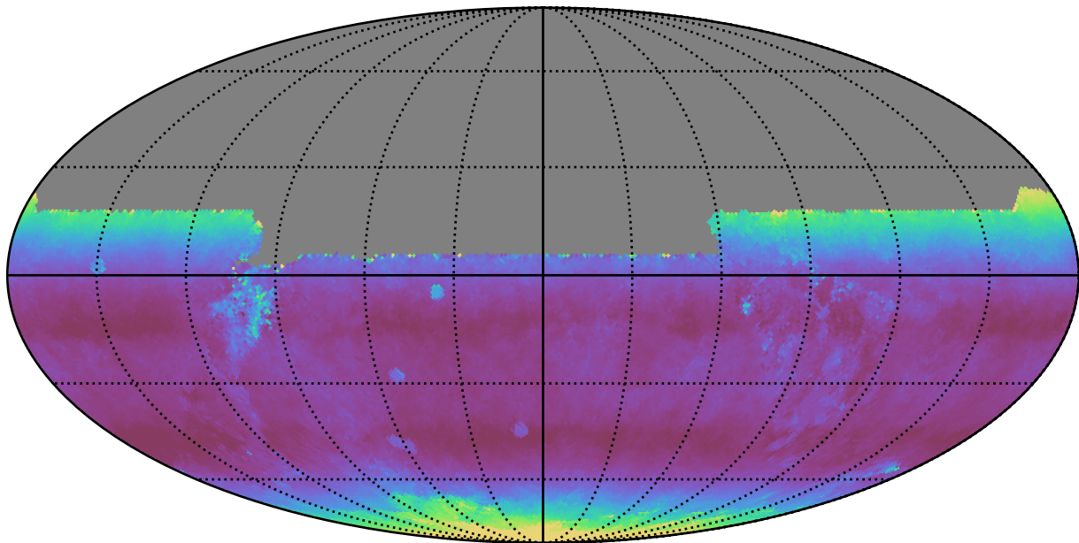
baseline_v3.5_10yrs All sky y band: Median airmass
