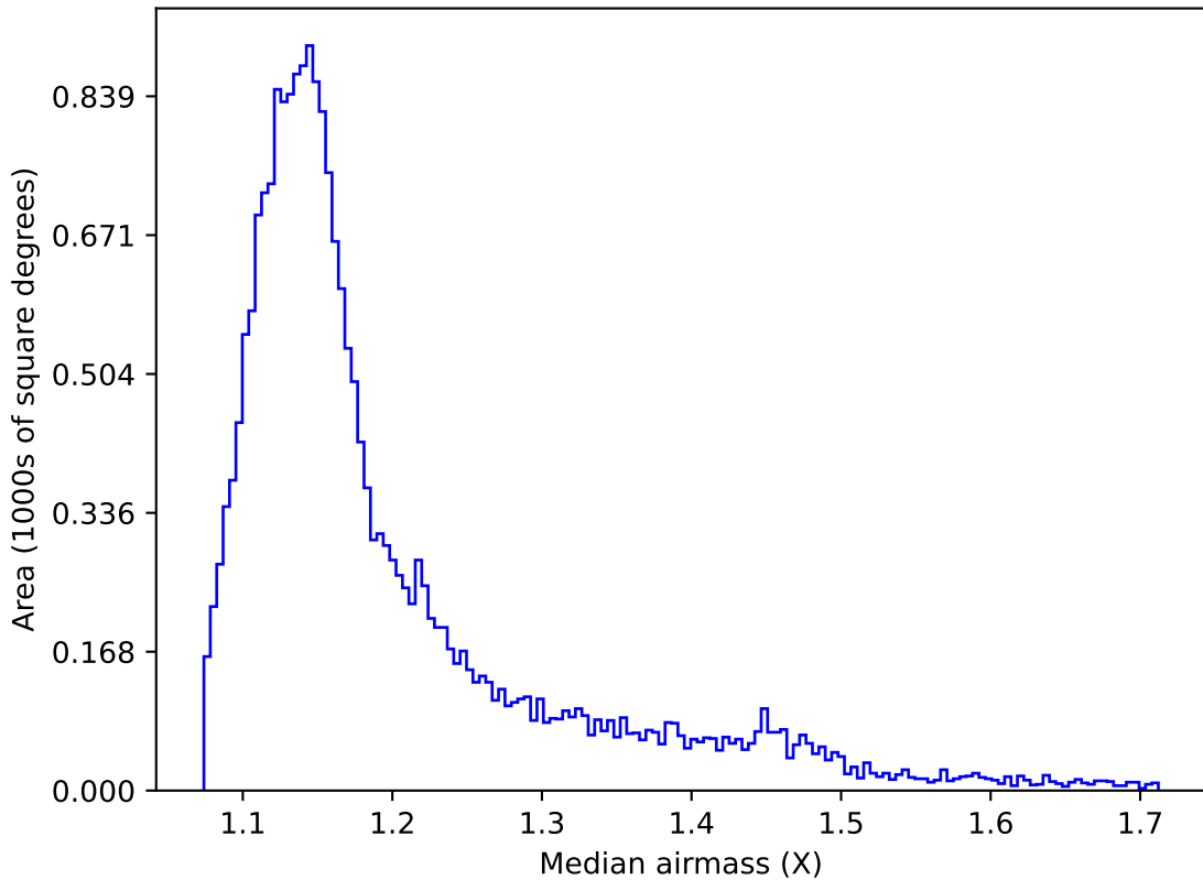
baseline_v3.5_10yrs All sky u band: Median airmass
