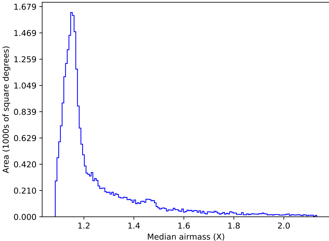
baseline_v3.5_10yrs All sky r band: Median airmass
