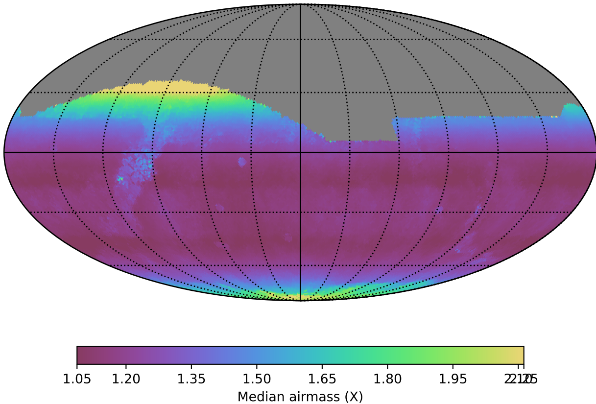
baseline_v3.5_10yrs All sky i band: Median airmass
