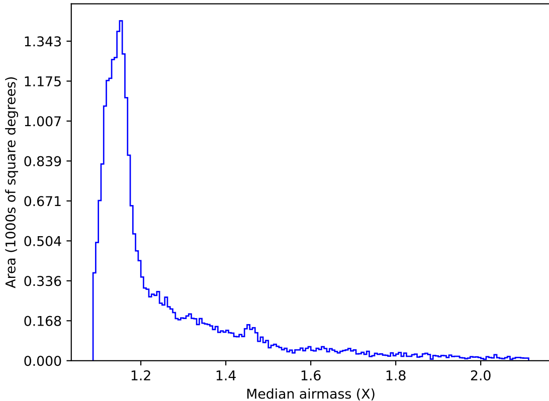
baseline_v3.5_10yrs All sky i band: Median airmass
