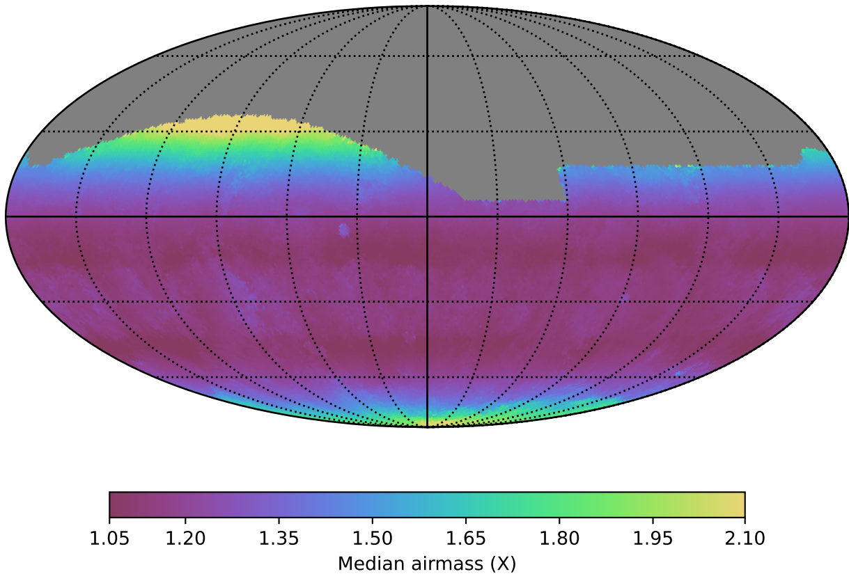
baseline_v3.5_10yrs All sky g band: Median airmass
