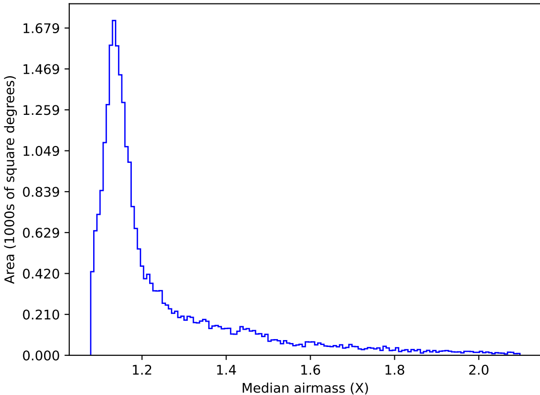
baseline_v3.5_10yrs All sky g band: Median airmass
