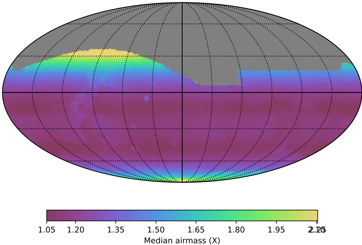
baseline_v3.5_10yrs All sky all bands: Median airmass
