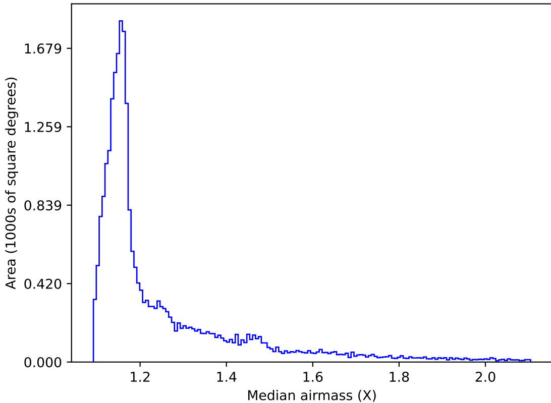
baseline_v3.5_10yrs All sky all bands: Median airmass
