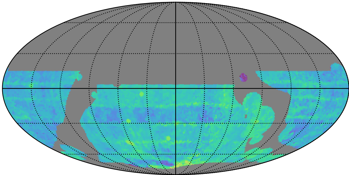
baseline_v3.5_10yrs WFD z band: Median Season Length
