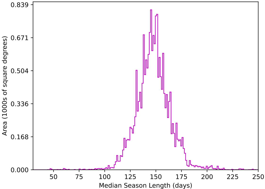
baseline_v3.5_10yrs WFD z band: Median Season Length
