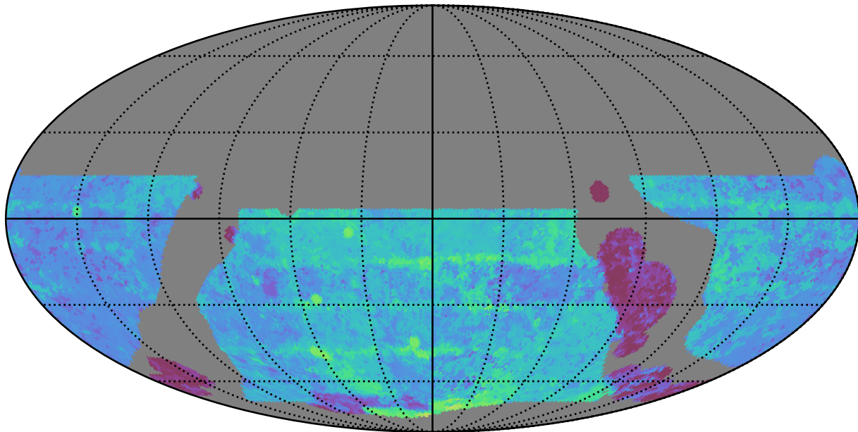
baseline_v3.5_10yrs WFD y band: Median Season Length
