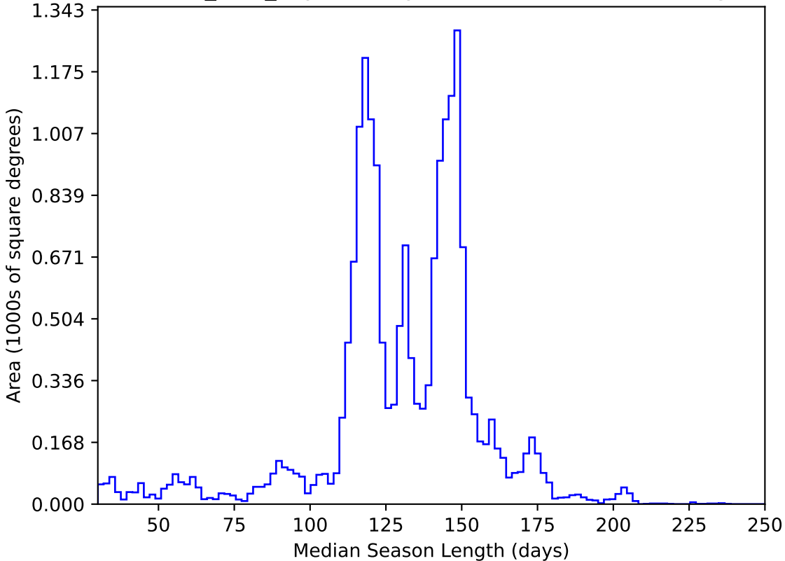
baseline_v3.5_10yrs WFD y band: Median Season Length
