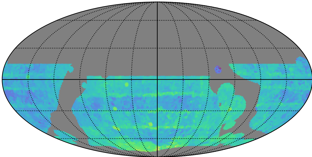
baseline_v3.5_10yrs WFD r band: Median Season Length
