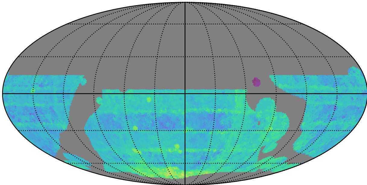
baseline_v3.5_10yrs WFD i band: Median Season Length
