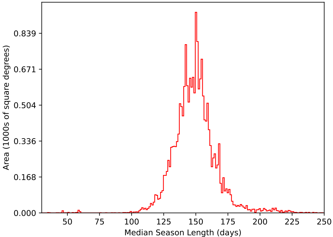
baseline_v3.5_10yrs WFD i band: Median Season Length
