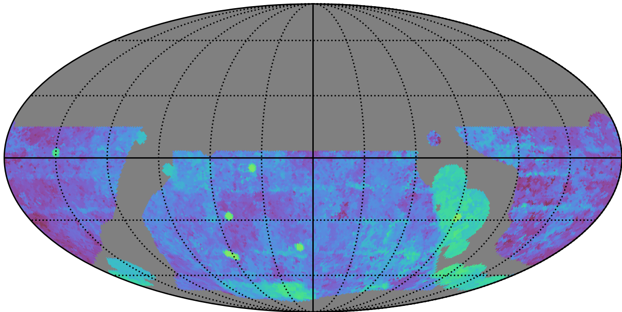
baseline_v3.5_10yrs WFD g band: Median Season Length
