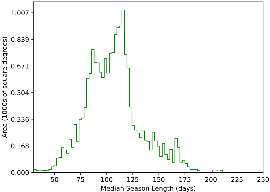
baseline_v3.5_10yrs WFD g band: Median Season Length
