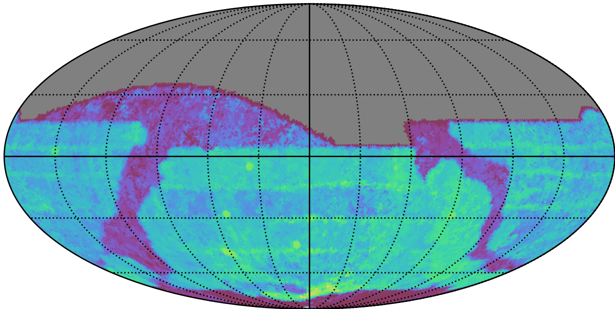
baseline_v3.5_10yrs All sky z band: Median Season Length
