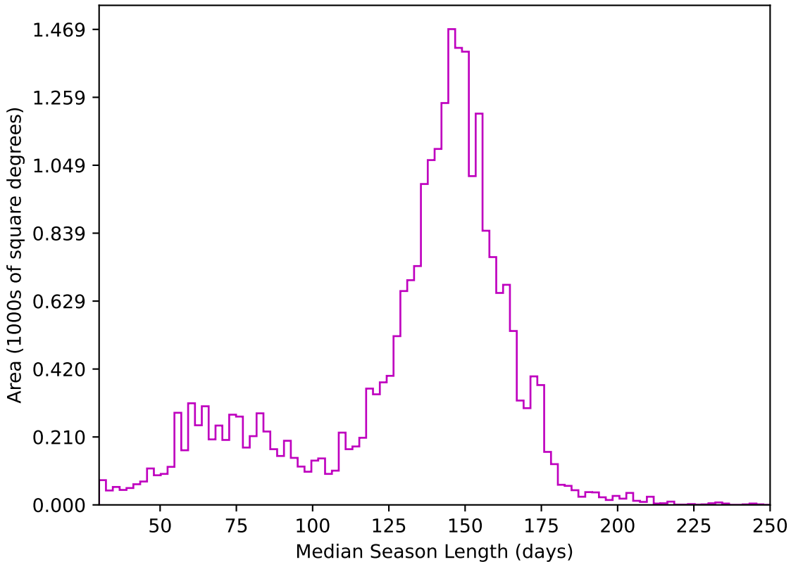
baseline_v3.5_10yrs All sky z band: Median Season Length
