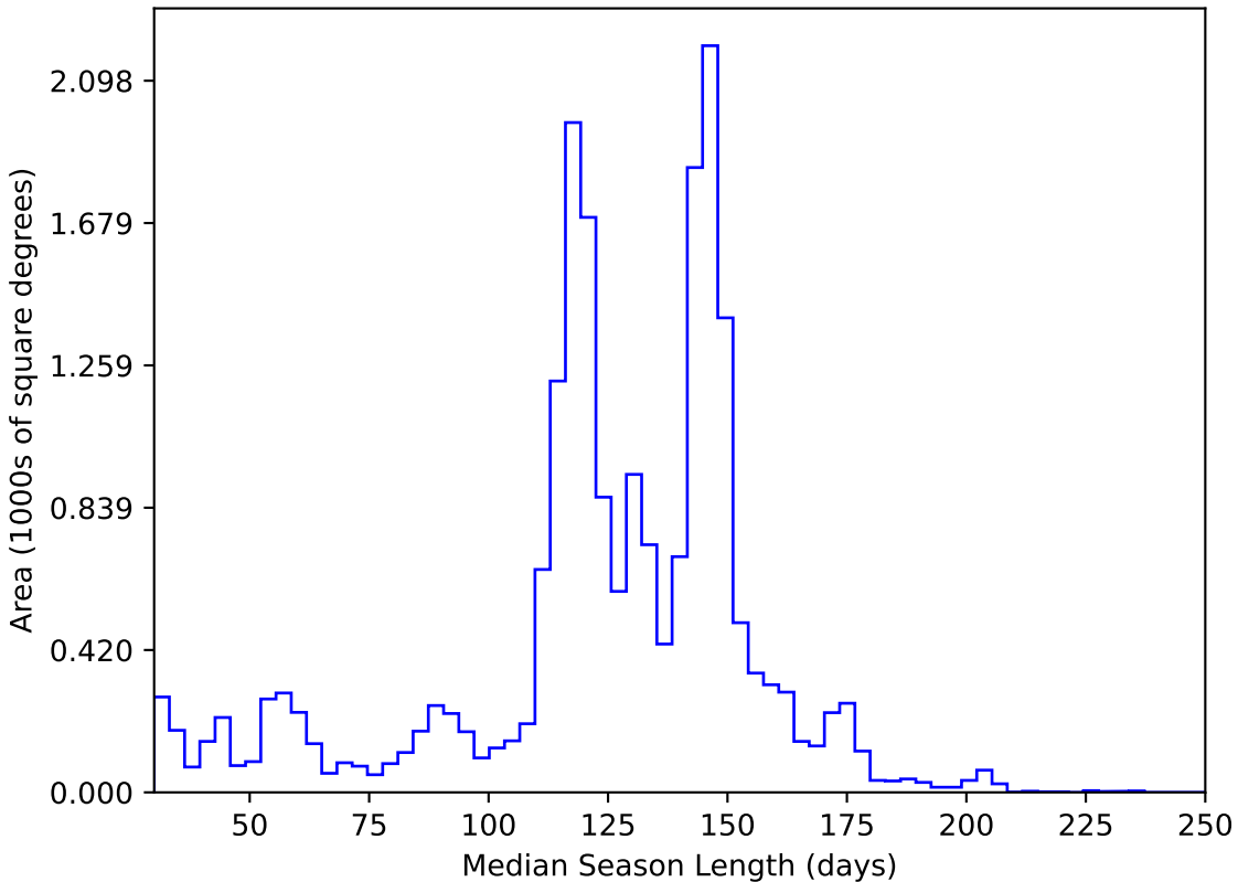
baseline_v3.5_10yrs All sky y band: Median Season Length
