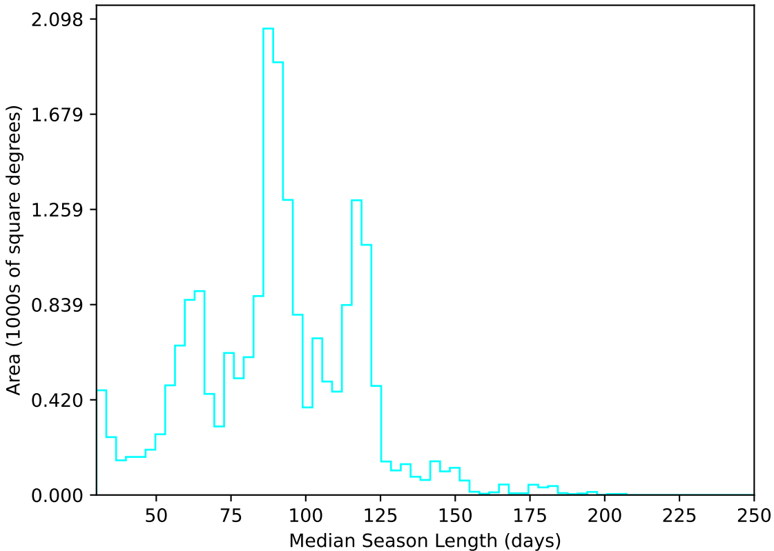
baseline_v3.5_10yrs All sky u band: Median Season Length
