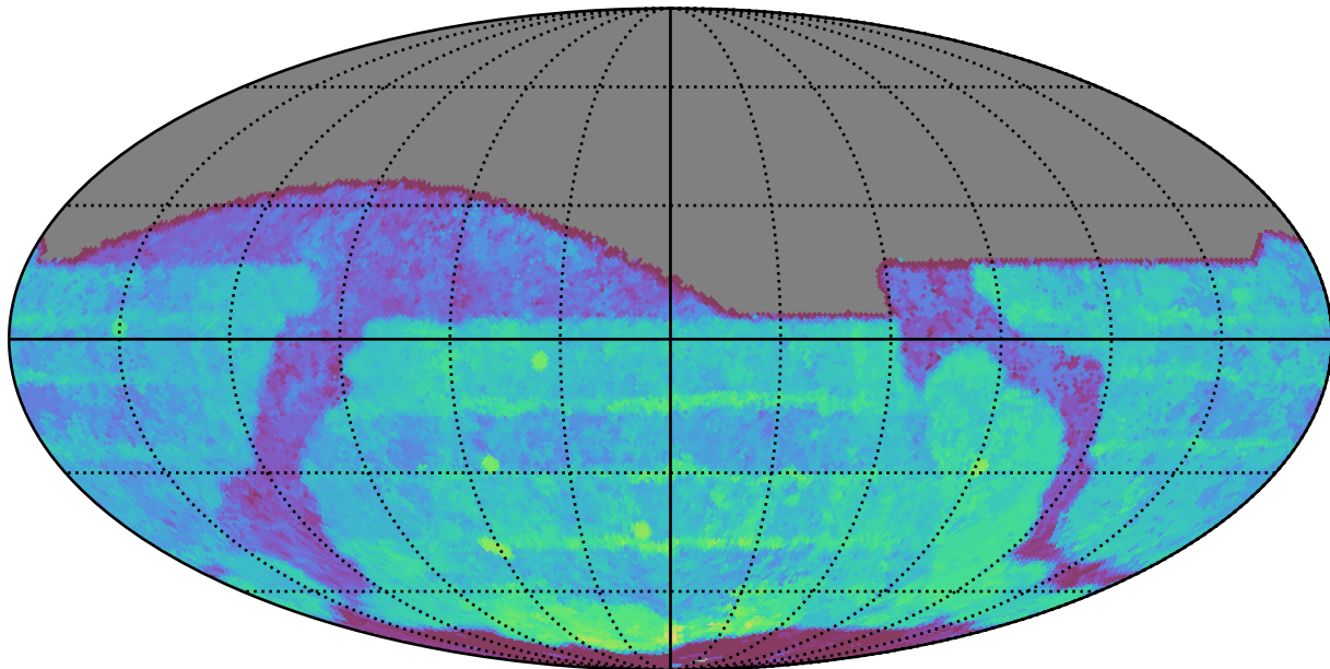
baseline_v3.5_10yrs All sky r band: Median Season Length
