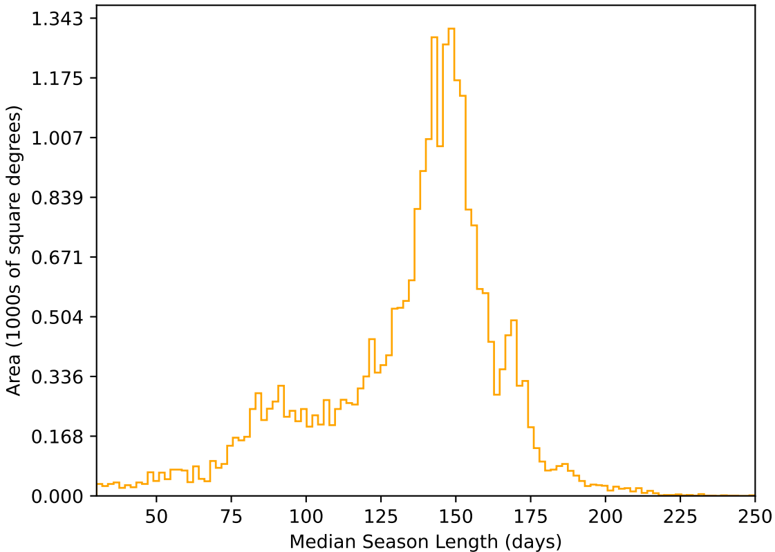
baseline_v3.5_10yrs All sky r band: Median Season Length
