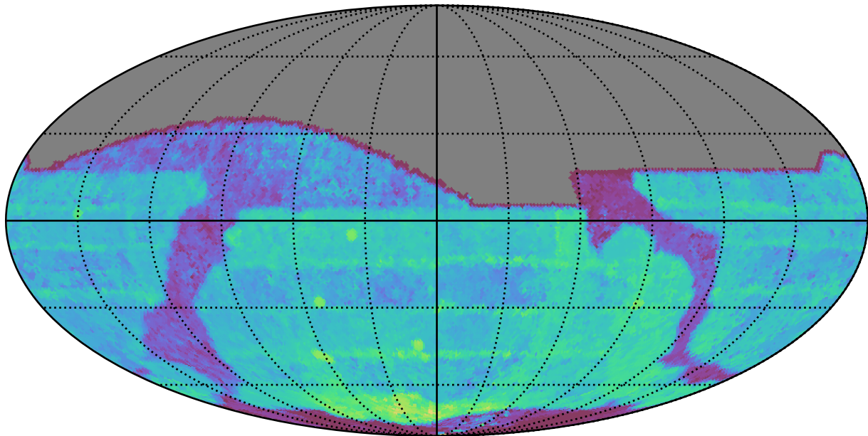
baseline_v3.5_10yrs All sky i band: Median Season Length
