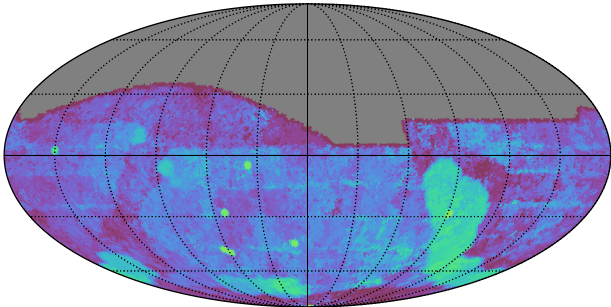
baseline_v3.5_10yrs All sky g band: Median Season Length
