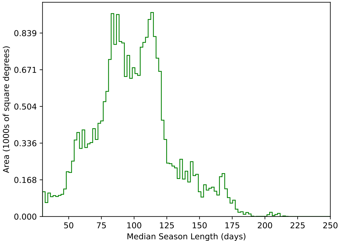
baseline_v3.5_10yrs All sky g band: Median Season Length
