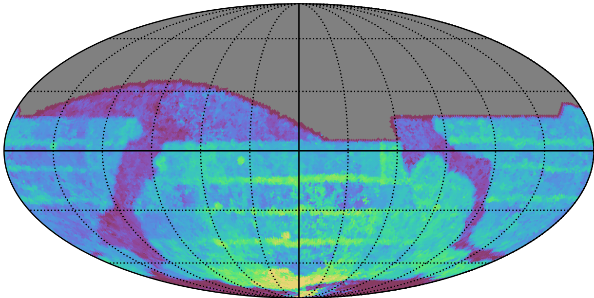
baseline_v3.5_10yrs All sky all bands: Median Season Length
