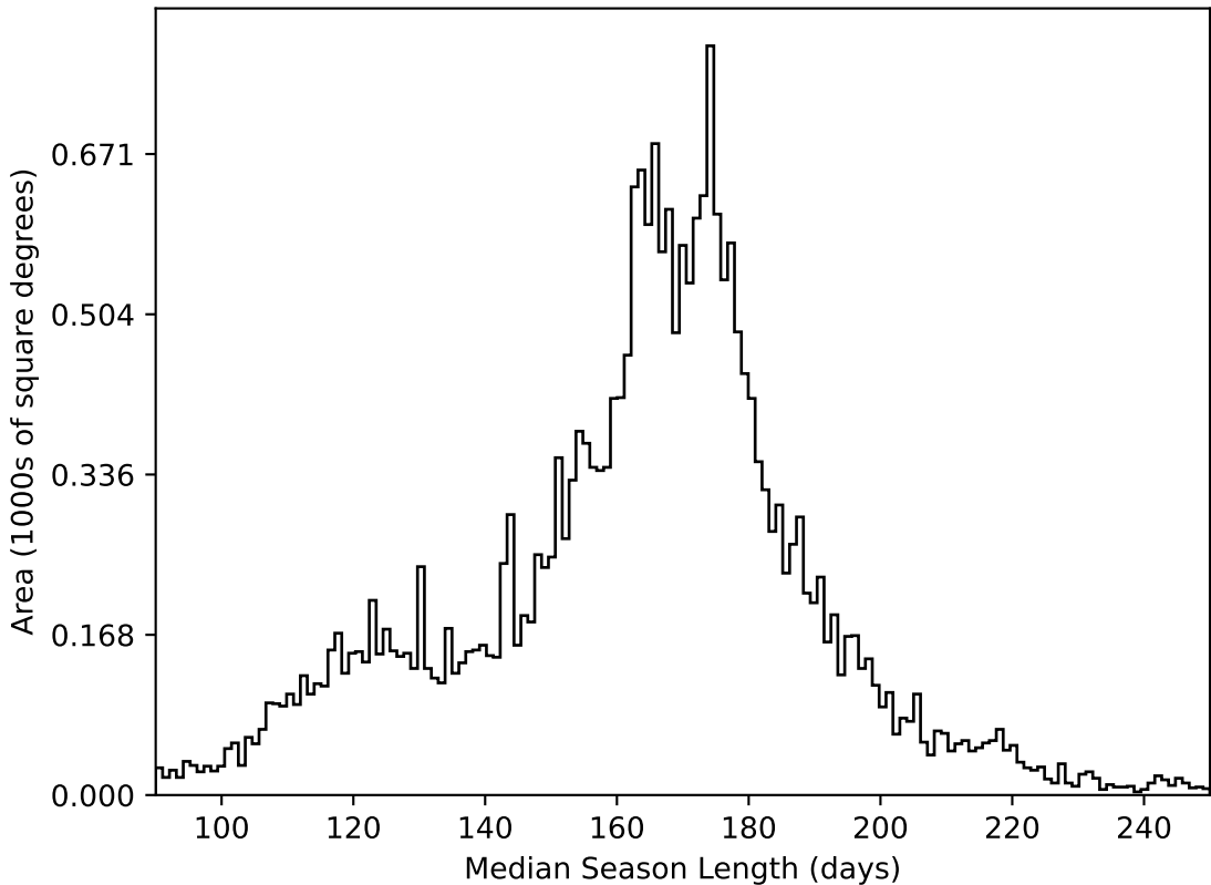
baseline_v3.5_10yrs All sky all bands: Median Season Length
