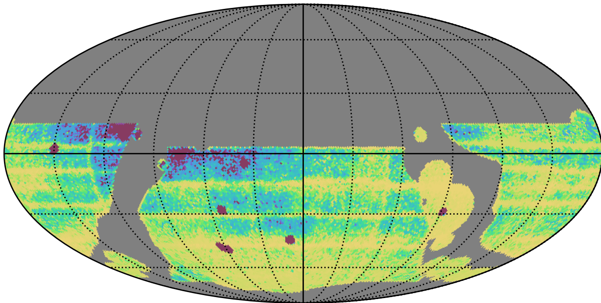
baseline_v3.5_10yrs WFD: Median Intra-Night Gap
