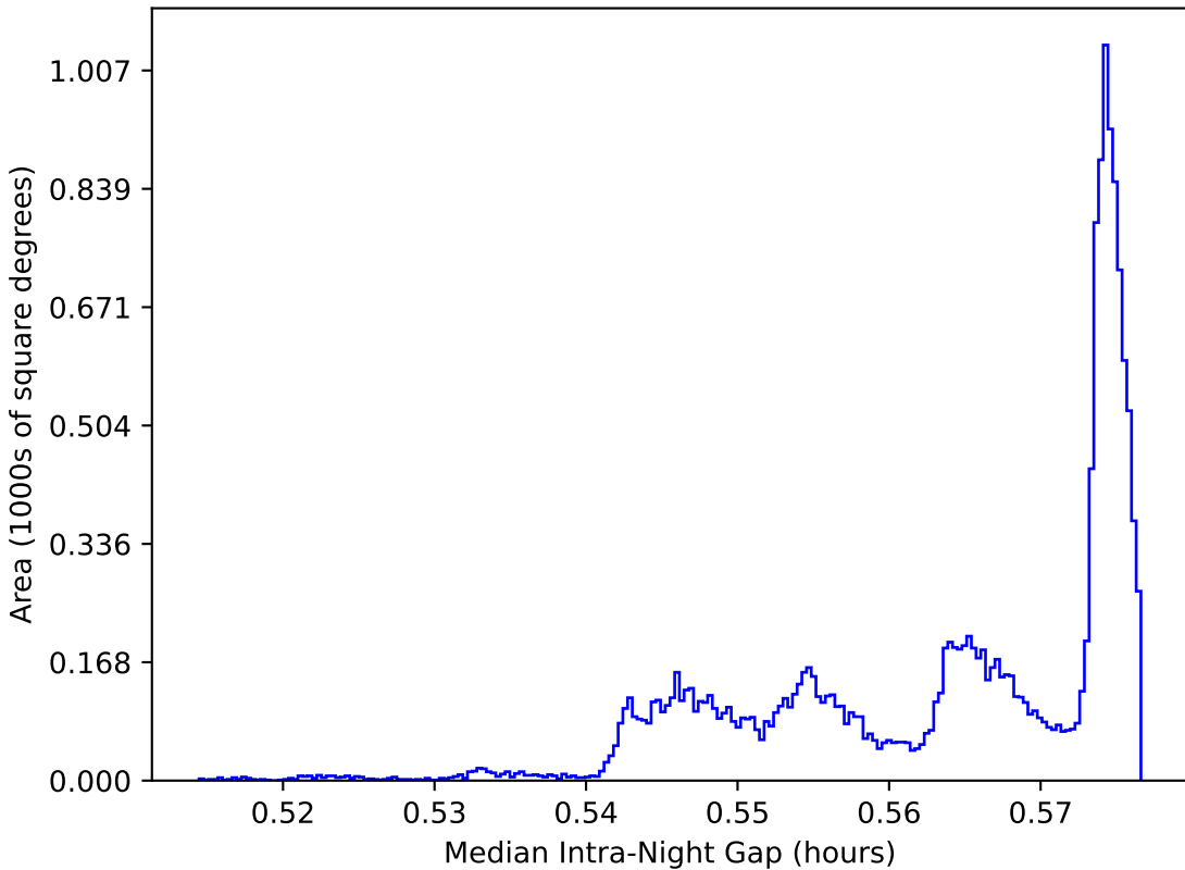
baseline_v3.5_10yrs WFD: Median Intra-Night Gap
