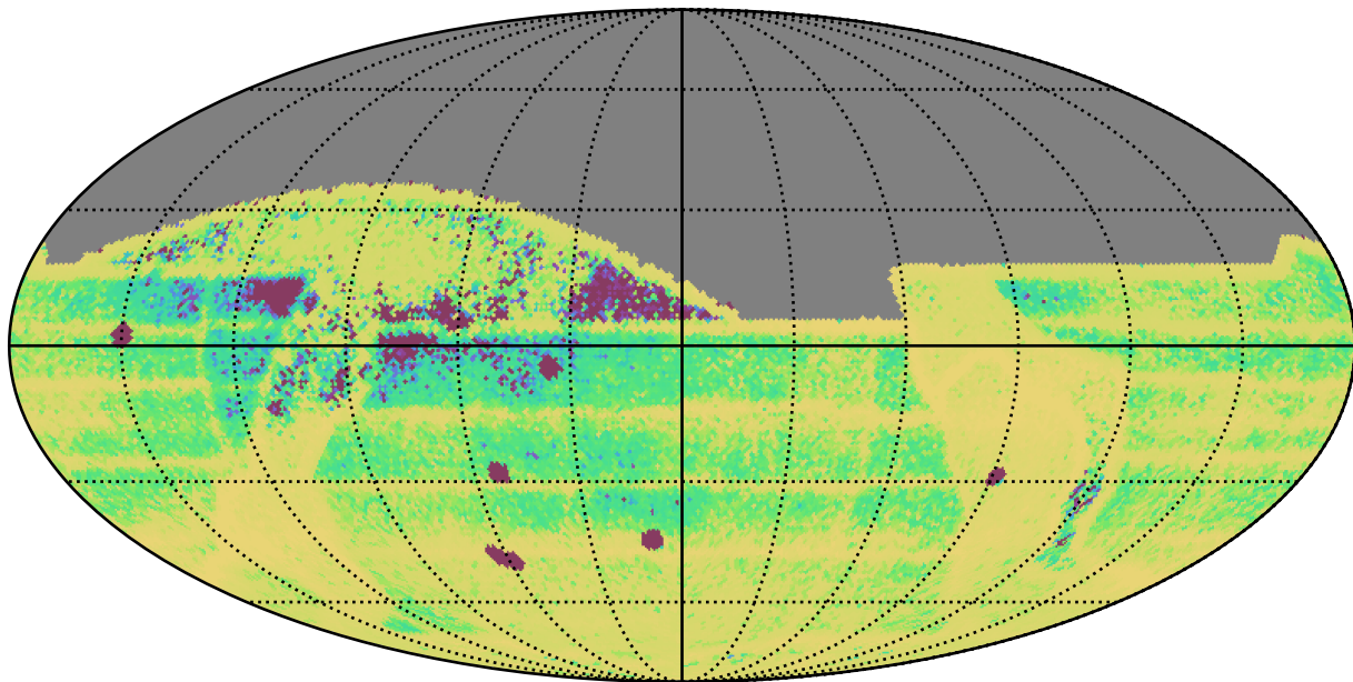
baseline_v3.5_10yrs All sky: Median Intra-Night Gap
