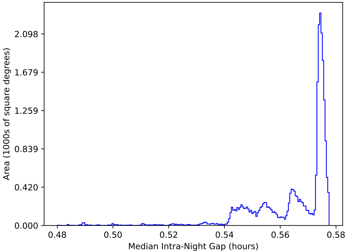
baseline_v3.5_10yrs All sky: Median Intra-Night Gap
