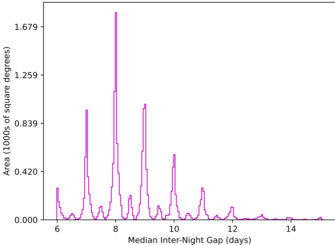
baseline_v3.5_10yrs WFD z band: Median Inter-Night Gap
