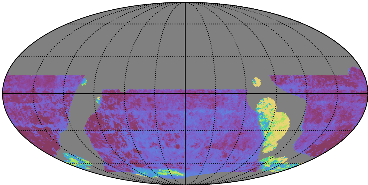
baseline_v3.5_10yrs WFD y band: Median Inter-Night Gap
