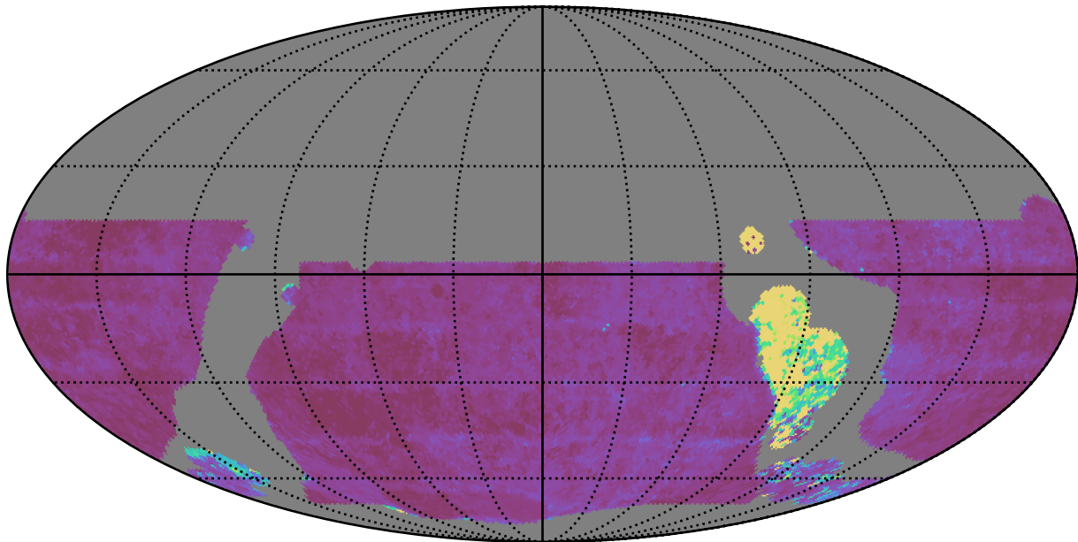
baseline_v3.5_10yrs WFD u band: Median Inter-Night Gap
