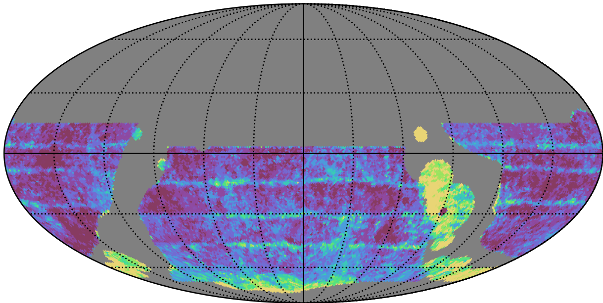
baseline_v3.5_10yrs WFD r band: Median Inter-Night Gap
