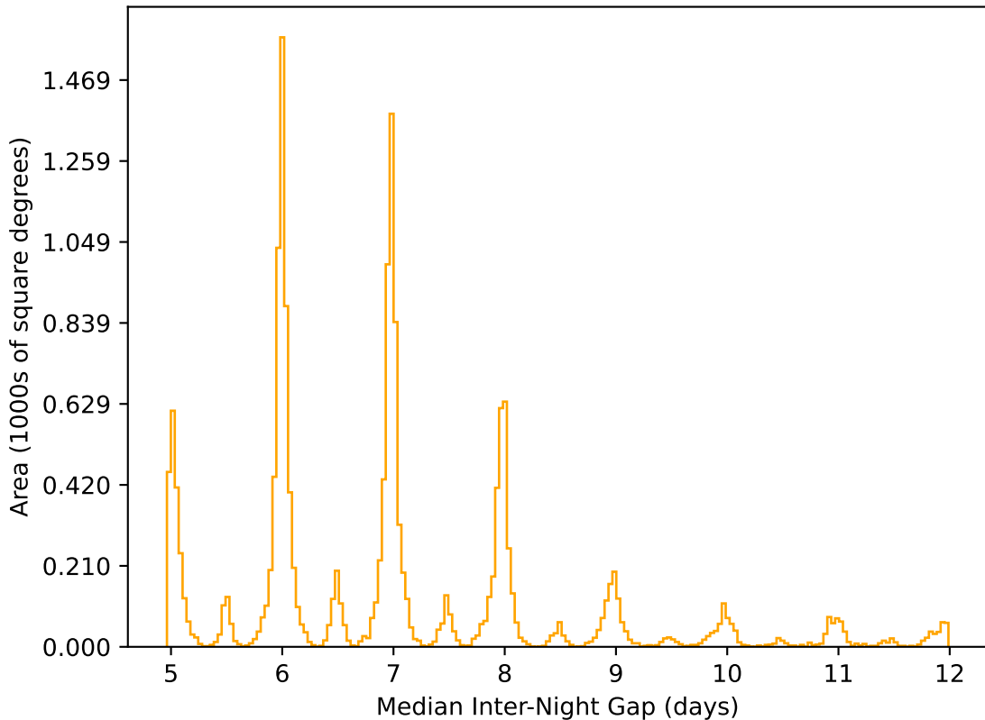
baseline_v3.5_10yrs WFD r band: Median Inter-Night Gap
