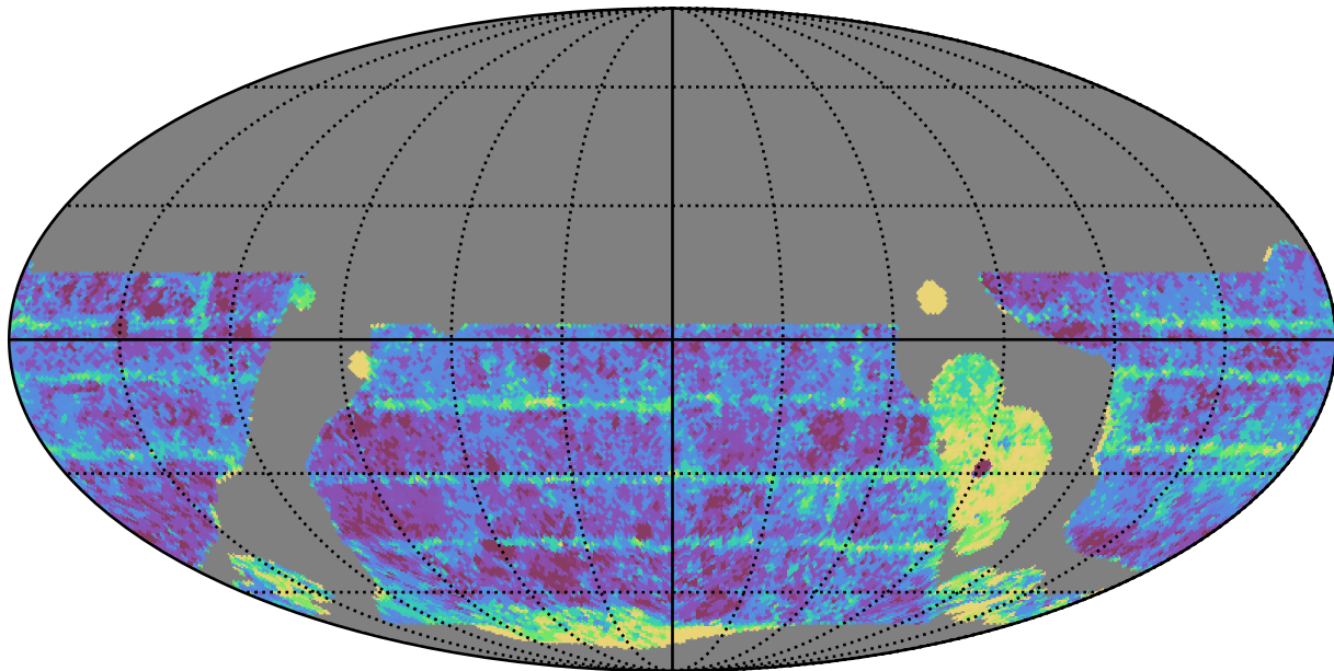
baseline_v3.5_10yrs WFD i band: Median Inter-Night Gap
