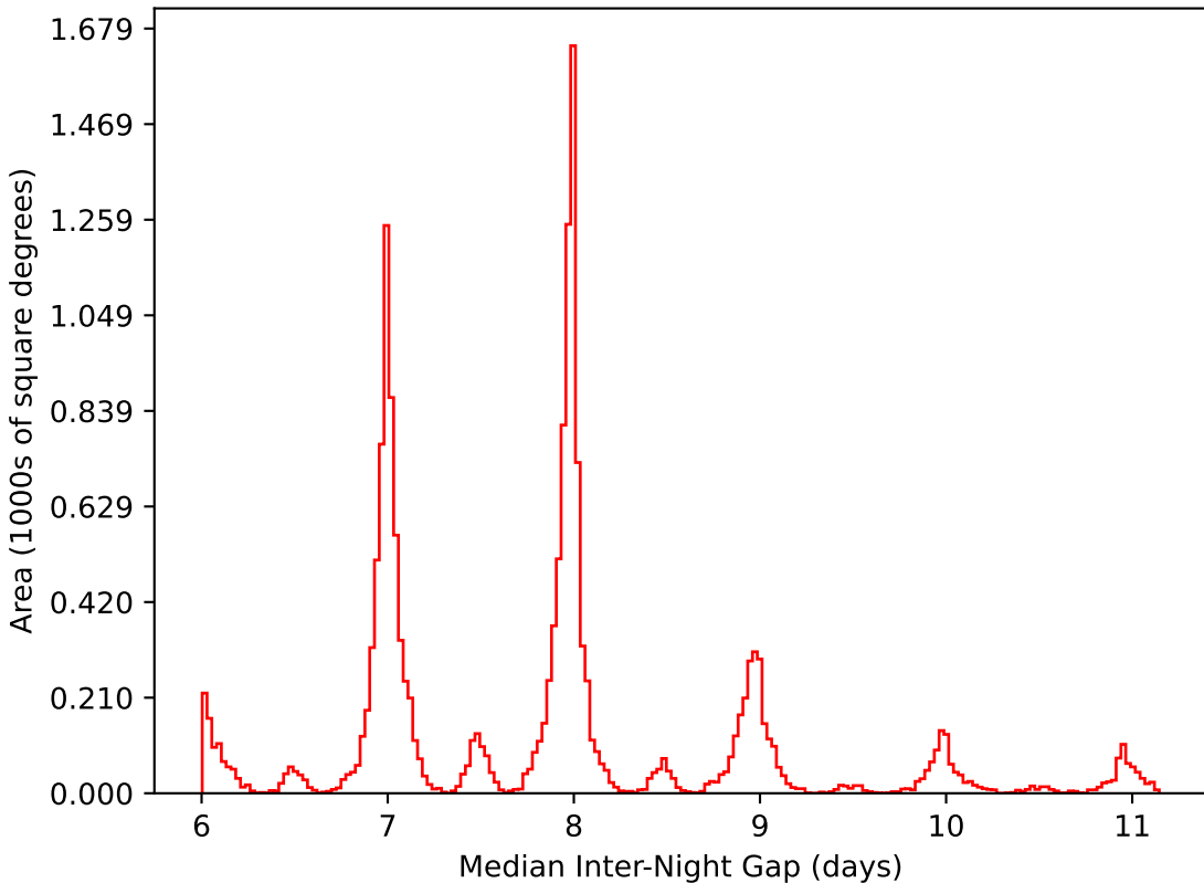
baseline_v3.5_10yrs WFD i band: Median Inter-Night Gap
