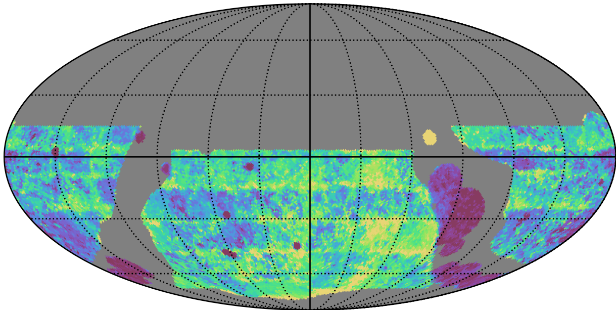
baseline_v3.5_10yrs WFD g band: Median Inter-Night Gap
