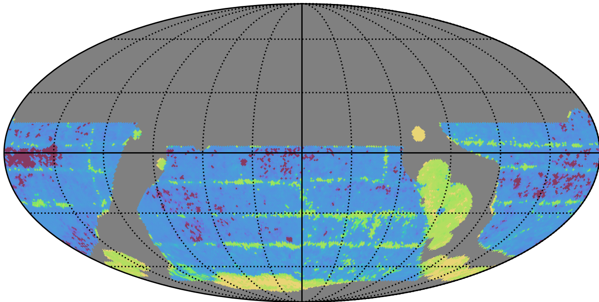
baseline_v3.5_10yrs WFD all bands: Median Inter-Night Gap
