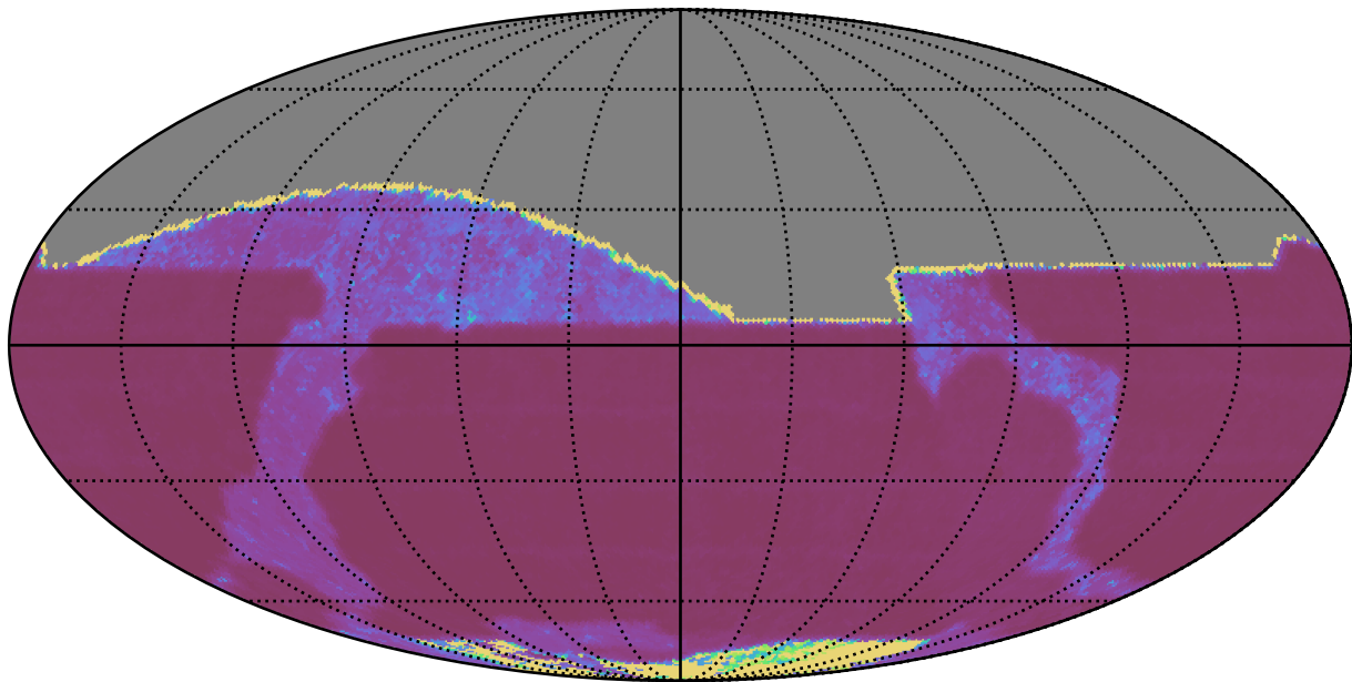
baseline_v3.5_10yrs All sky z band: Median Inter-Night Gap
