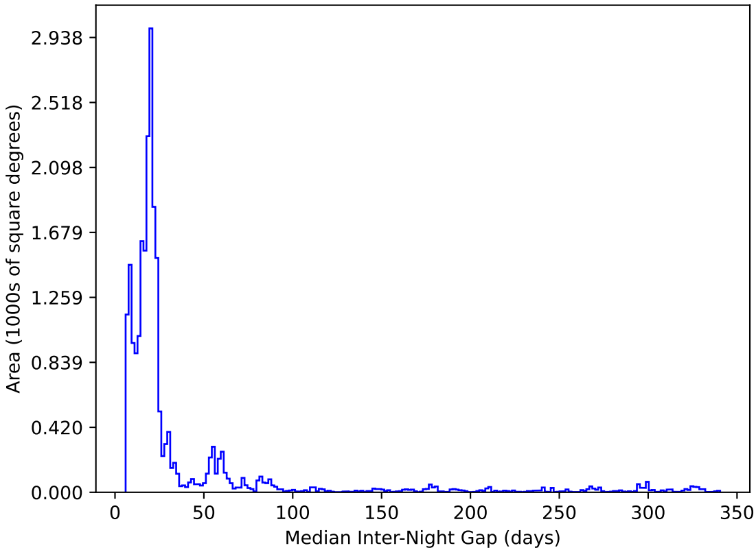
baseline_v3.5_10yrs All sky y band: Median Inter-Night Gap
