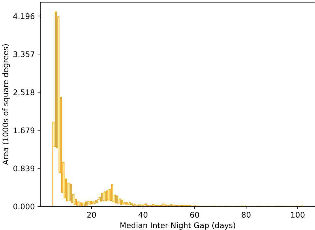
baseline_v3.5_10yrs All sky r band: Median Inter-Night Gap
