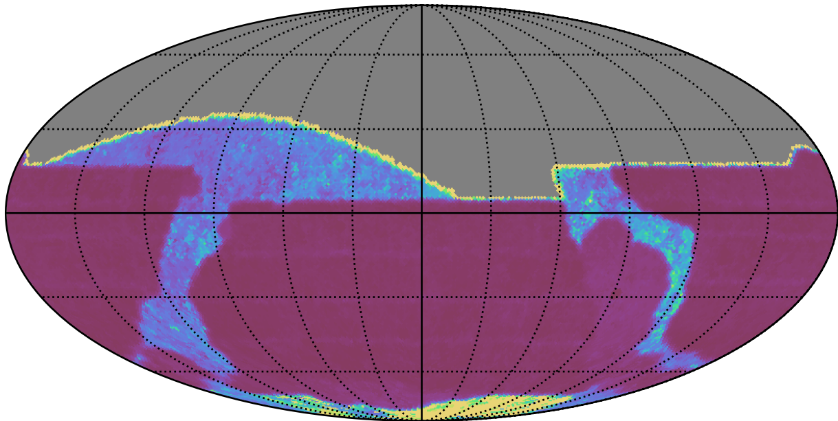
baseline_v3.5_10yrs All sky i band: Median Inter-Night Gap
