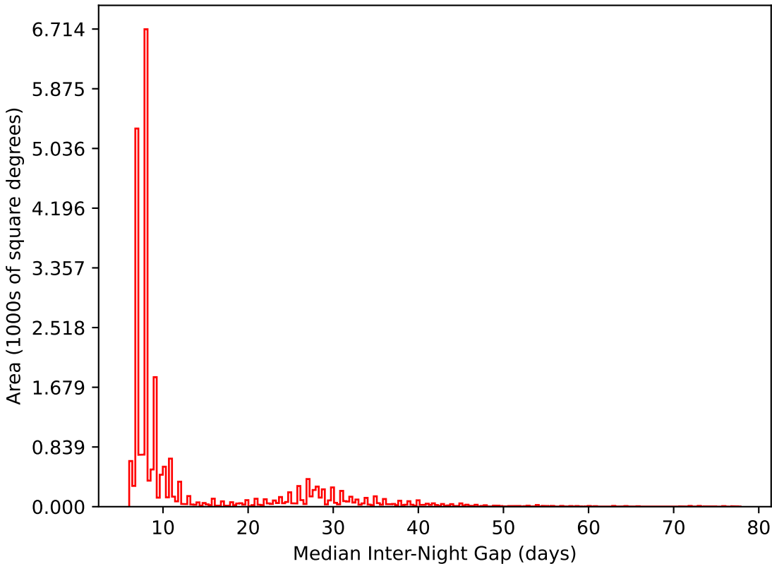
baseline_v3.5_10yrs All sky i band: Median Inter-Night Gap
