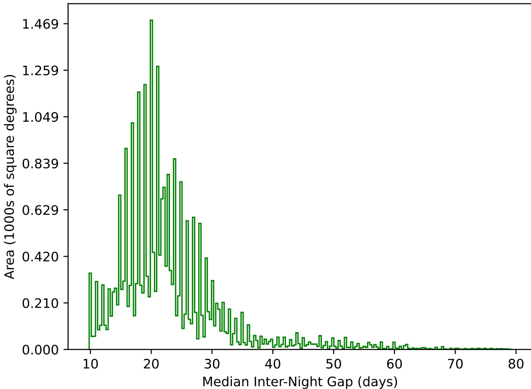
baseline_v3.5_10yrs All sky g band: Median Inter-Night Gap
